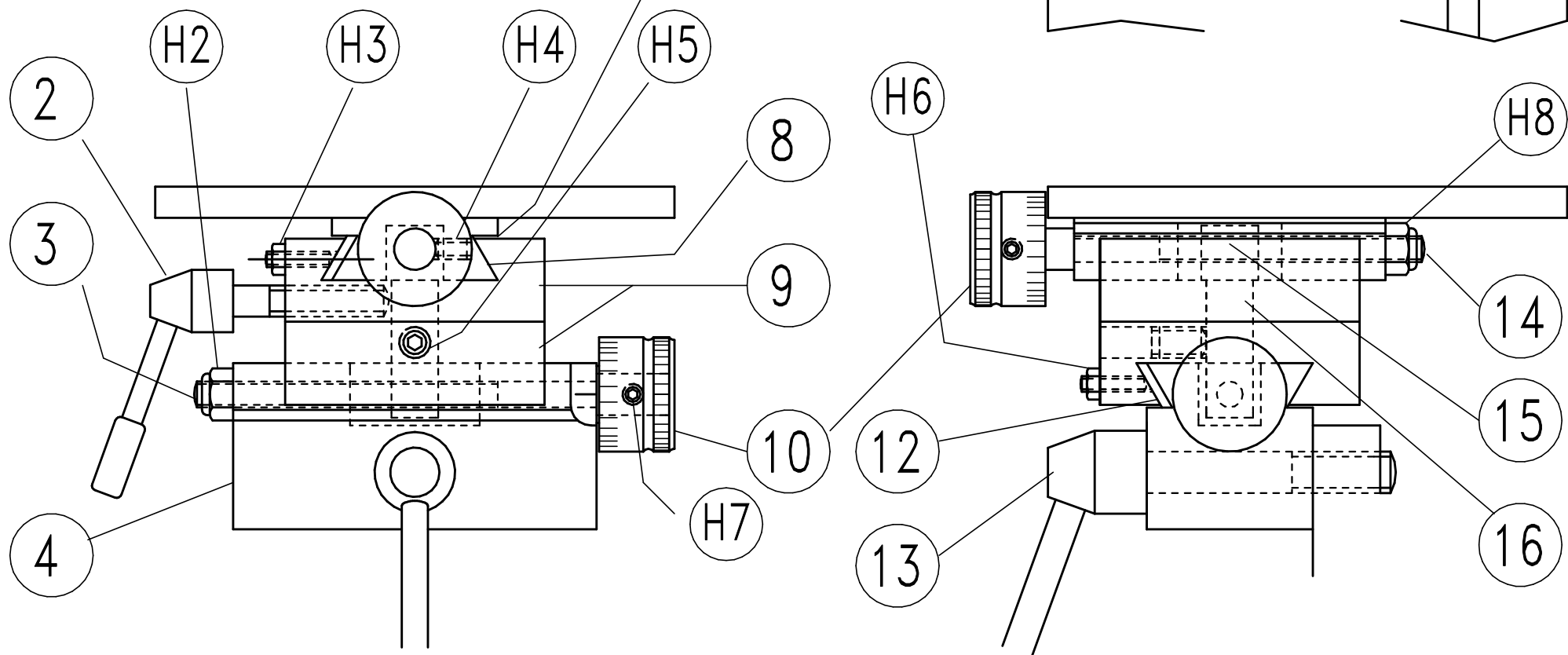
GRINDING REST PART ASSEMBLY
